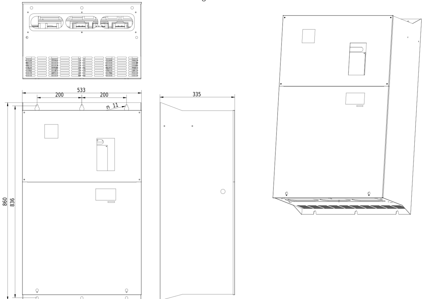
Dimensional drawing V810 - 250kW 4T2500
