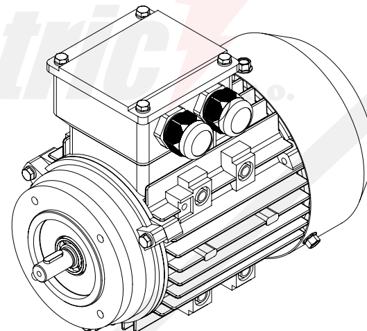
1AL-63-B14 Mounting diagram
